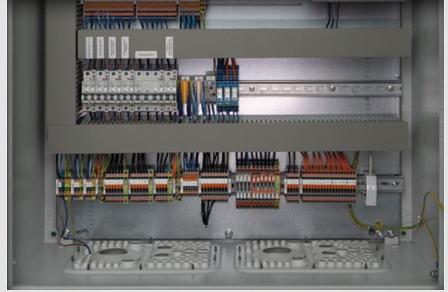
Customer-specific transfer terminal block
